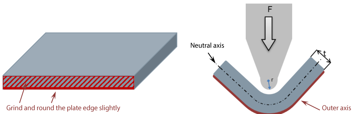
Graphic 3 Bending
