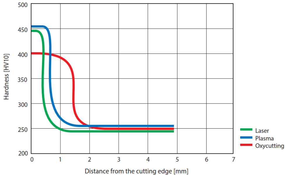
Graphic 4 Typical effect of different flame cutting processes on the hardness of the heat affected zone of a water quenched, fine grained structural steel with a yield strength of 690 MPa
