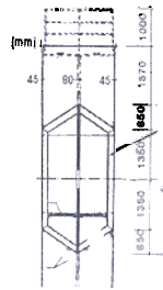
Fig. 5.5.6: Cross section of tension ties made of S460 TM
